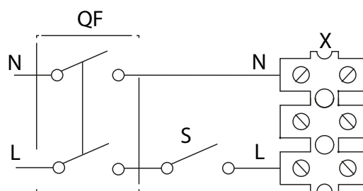
Diagram 3 Connection of the Duo fan to power mains
