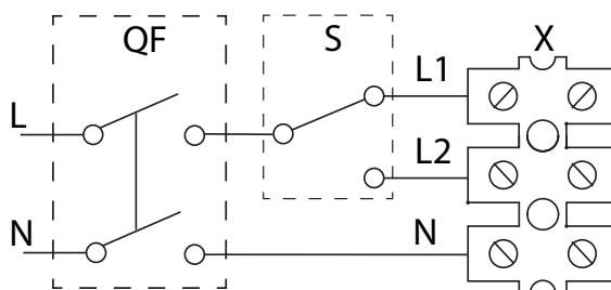
Diagram 3 Connection of the Duo fan to power mains
