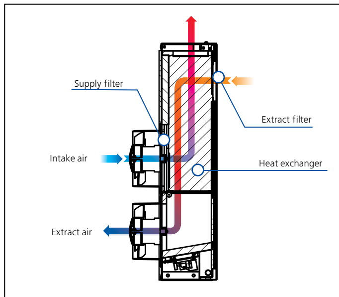
Fig. 2. Operation logic
