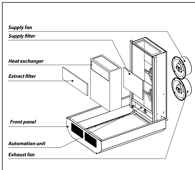
Fig. 1. Unit design
